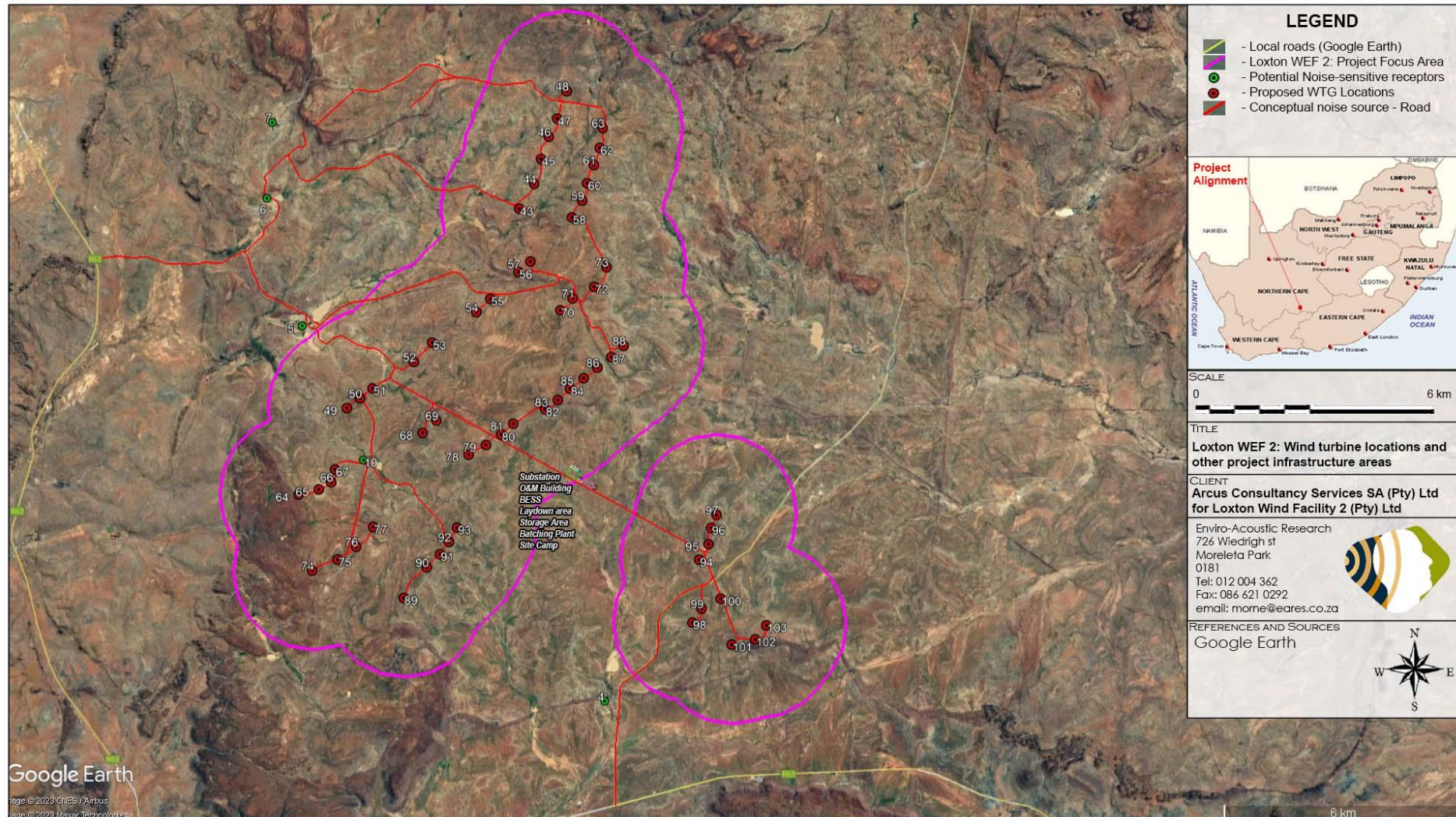
Figure 9-1: WTG locations and associated infrastructure for the proposed Loxton WEF 2
