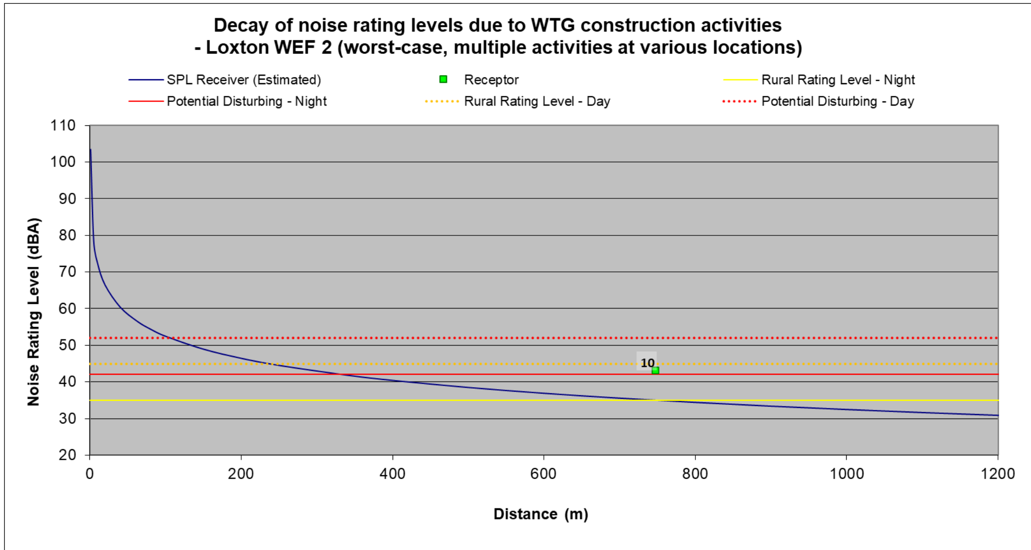
Figure 9-3: Projected conceptual construction noise levels for the proposed Loxton WEF 2
