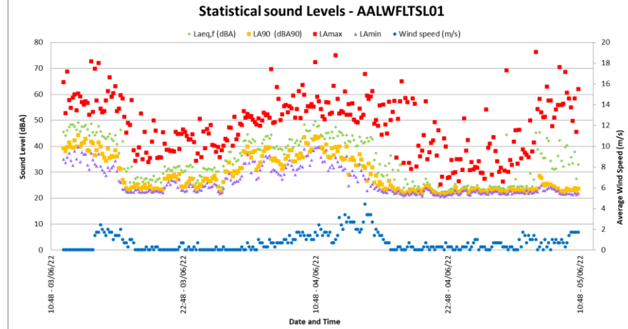
Figure 4-6: Maximum, minimum and Statistical sound levels at AALWFTSL01
