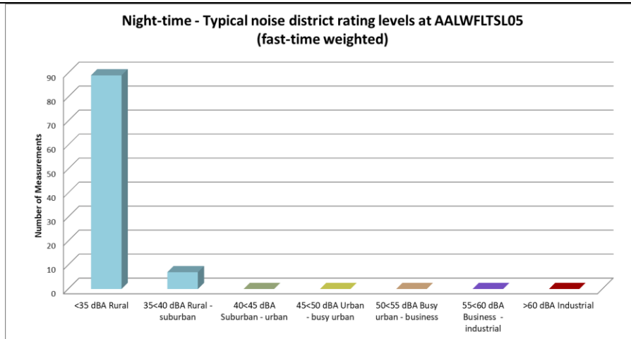
Figure 4-23: Classification of night-time measurements in typical noise districts at AALWFTSL05
