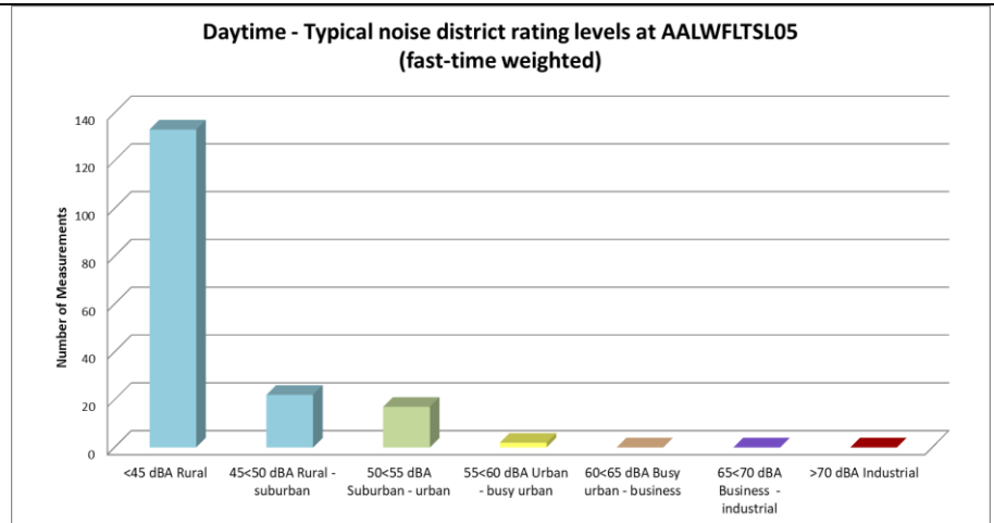
Figure 4-24: Classification of daytime measurements in typical noise districts at AALWFTSL05
