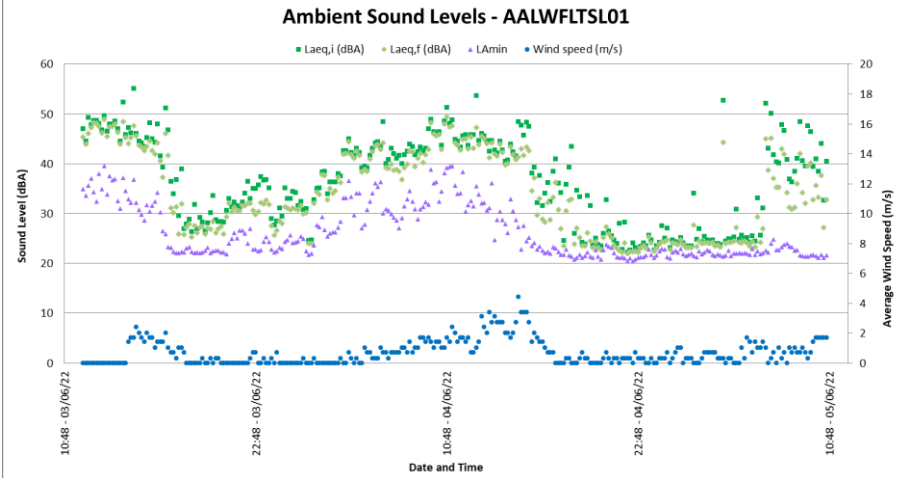
Figure 4-5: Ambient Sound Levels at AALWFTSL01
