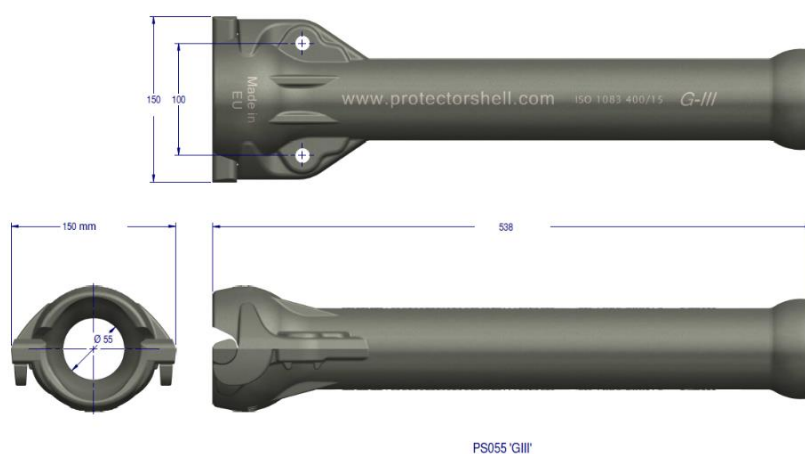
Figure 2-24 Example of Articulated Pipe
