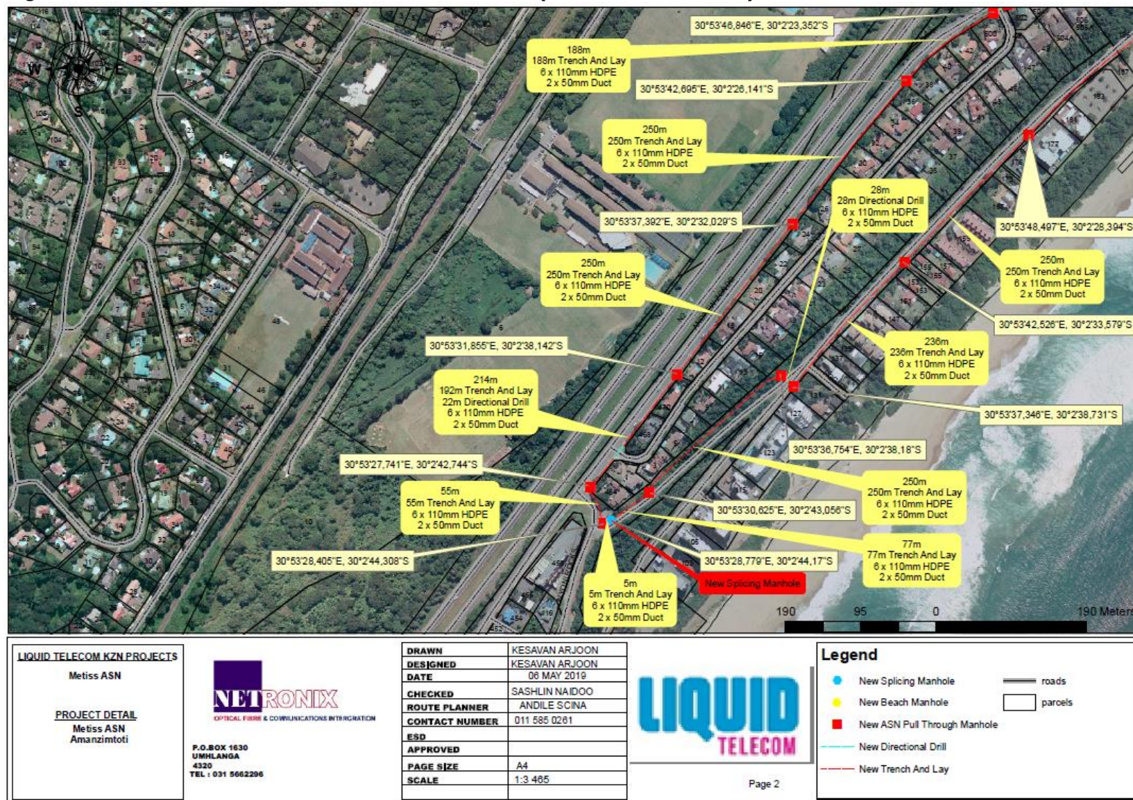
Figure 3-5 Section of the Terrestrial Cable Route 2 (Preferred)
