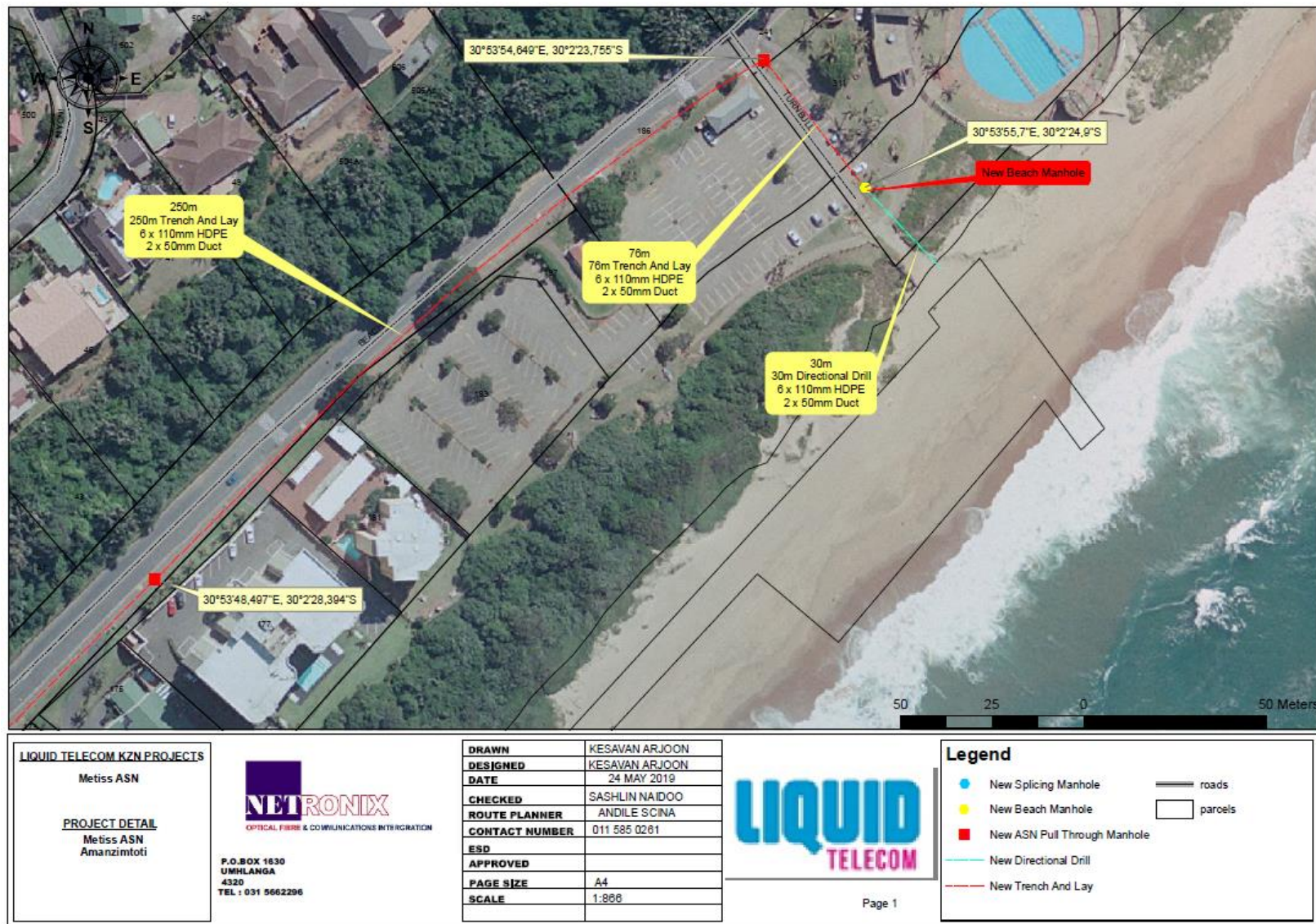
Figure 3-3 Section of the Terrestrial Cable Route 2 (Preferred, as presented in the Scoping Report)
