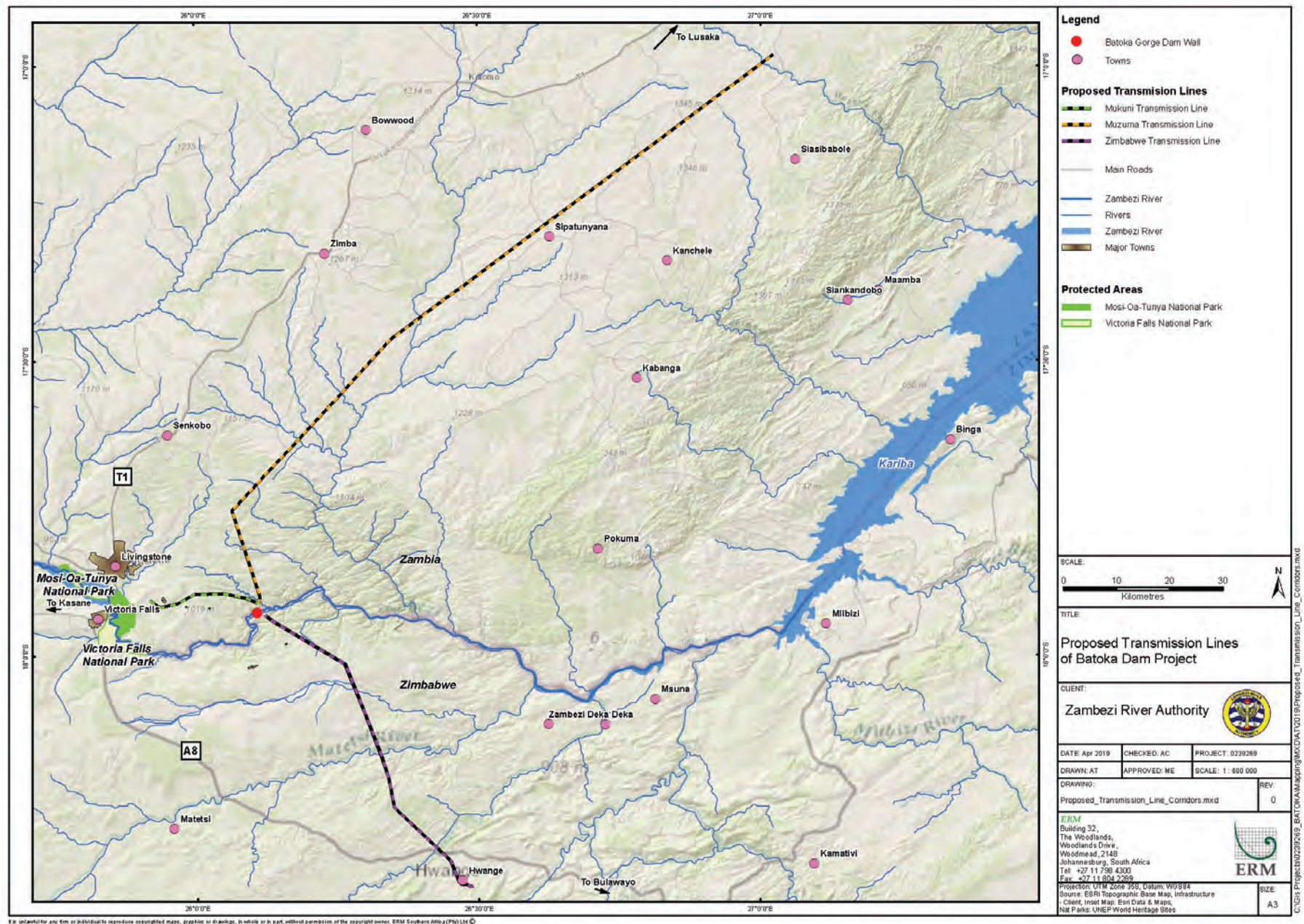
Figure 1.3 Proposed Transmission Line Routes
