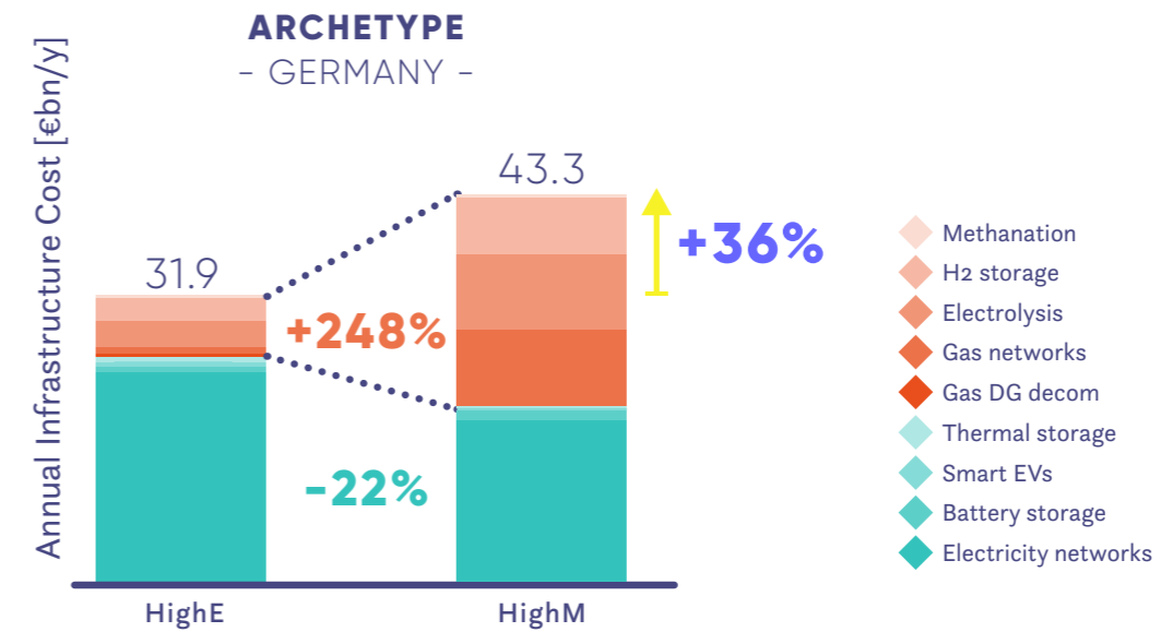
FIGURE 11: Infrastructure investments in HighE and HighM
