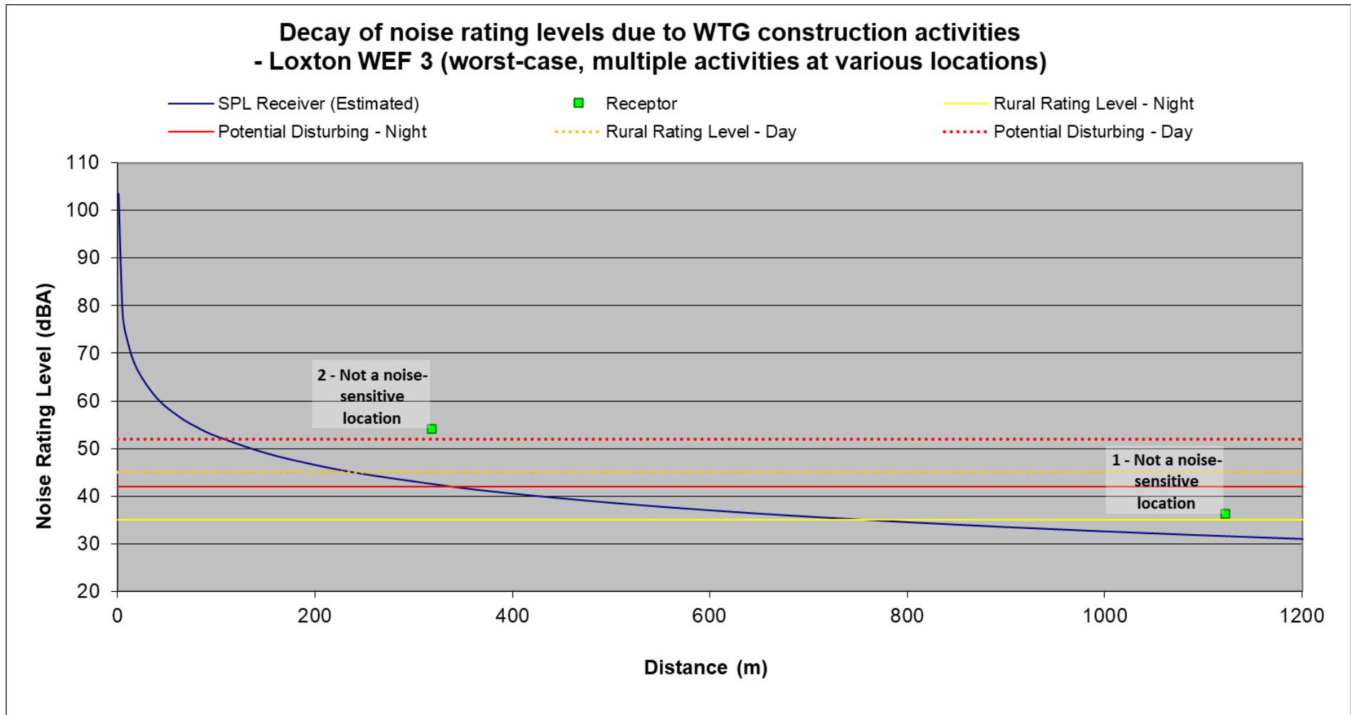
Figure 9-3: Projected conceptual construction noise levels for the proposed Loxton WEF 3
