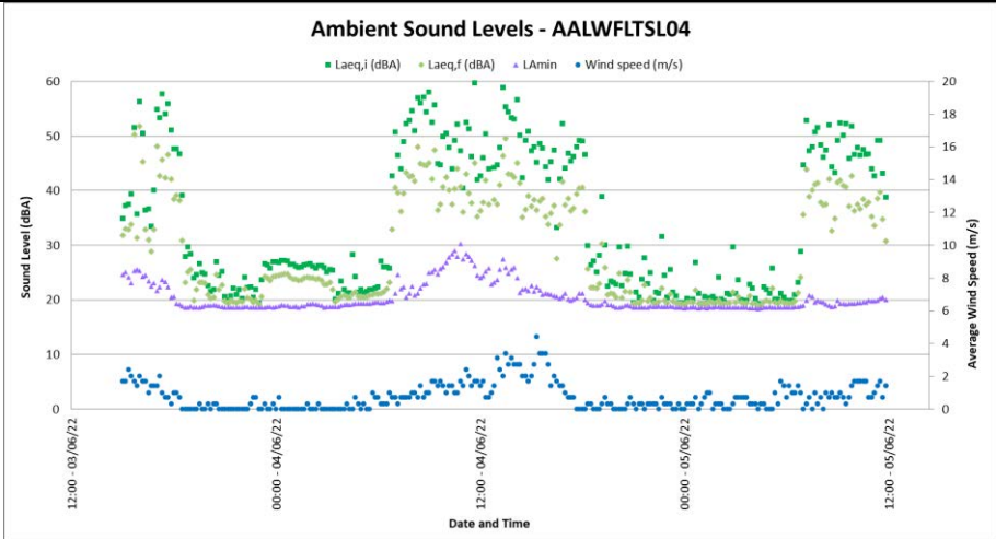
Figure 4-17: Ambient Sound Levels at AALWFTSL04
