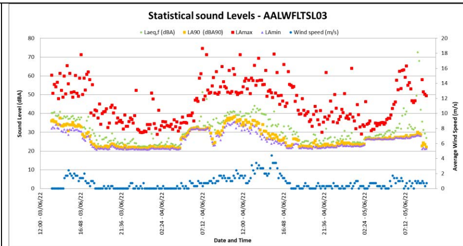
Figure 4-14: Maximum, minimum and Statistical sound levels at AALWFLTSLO3
