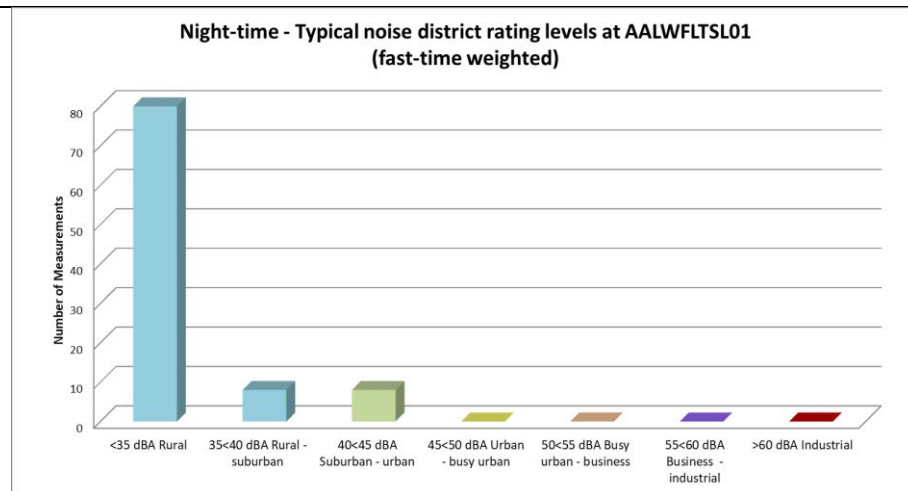
Figure 4-7: Classification of night-time measurements in typical noise districts at AALWFLTSLO1
