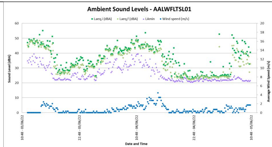
Figure 4-5: Ambient Sound Levels at AALWFLTSLO1
