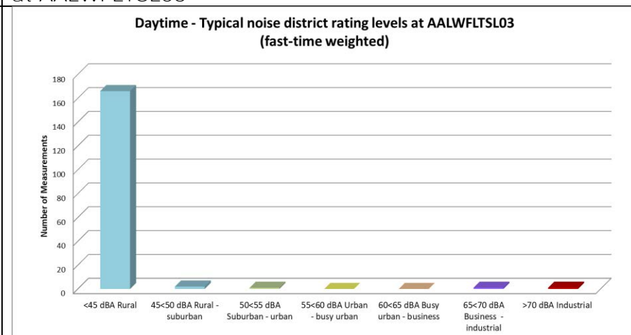
Figure 4-16: Classification of daytime measurements in typical noise districts at AALWFLTSLO3
