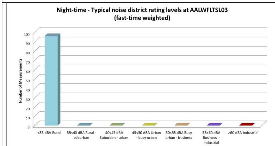
Figure 4-15: Classification of night-time measurements in typical noise districts at AALWFLTSLO3
