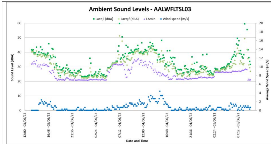
Figure 4-13: Ambient Sound Levels at AALWFLTSLO3
