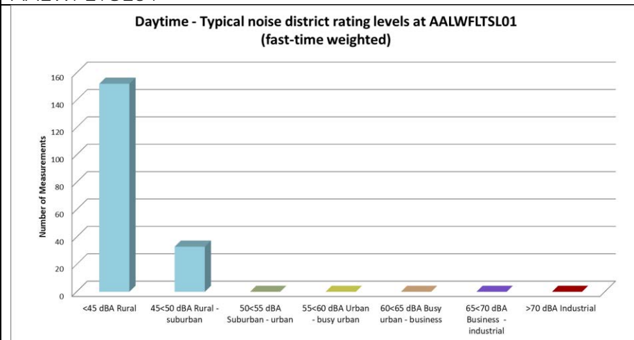
Figure 4-8: Classification of daytime measurements in typical noise districts at AALWFLTSLO1
