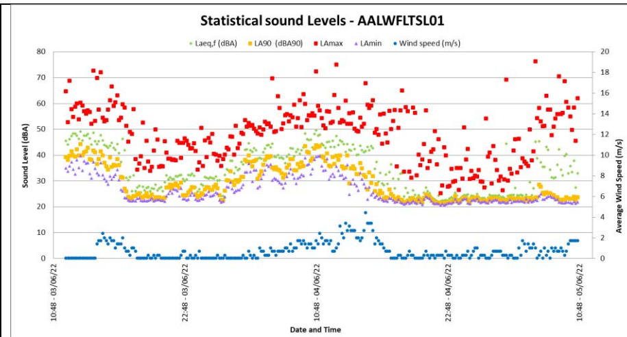
Figure 4-6: Maximum, minimum and Statistical sound levels at AALWFLTSLO1
