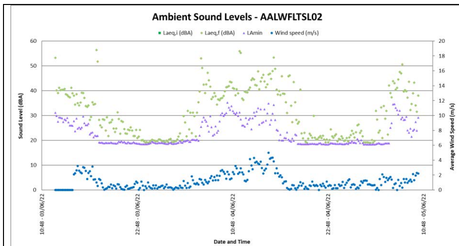
Figure 4-9: Ambient sound levels at AALWFLTSLO2
